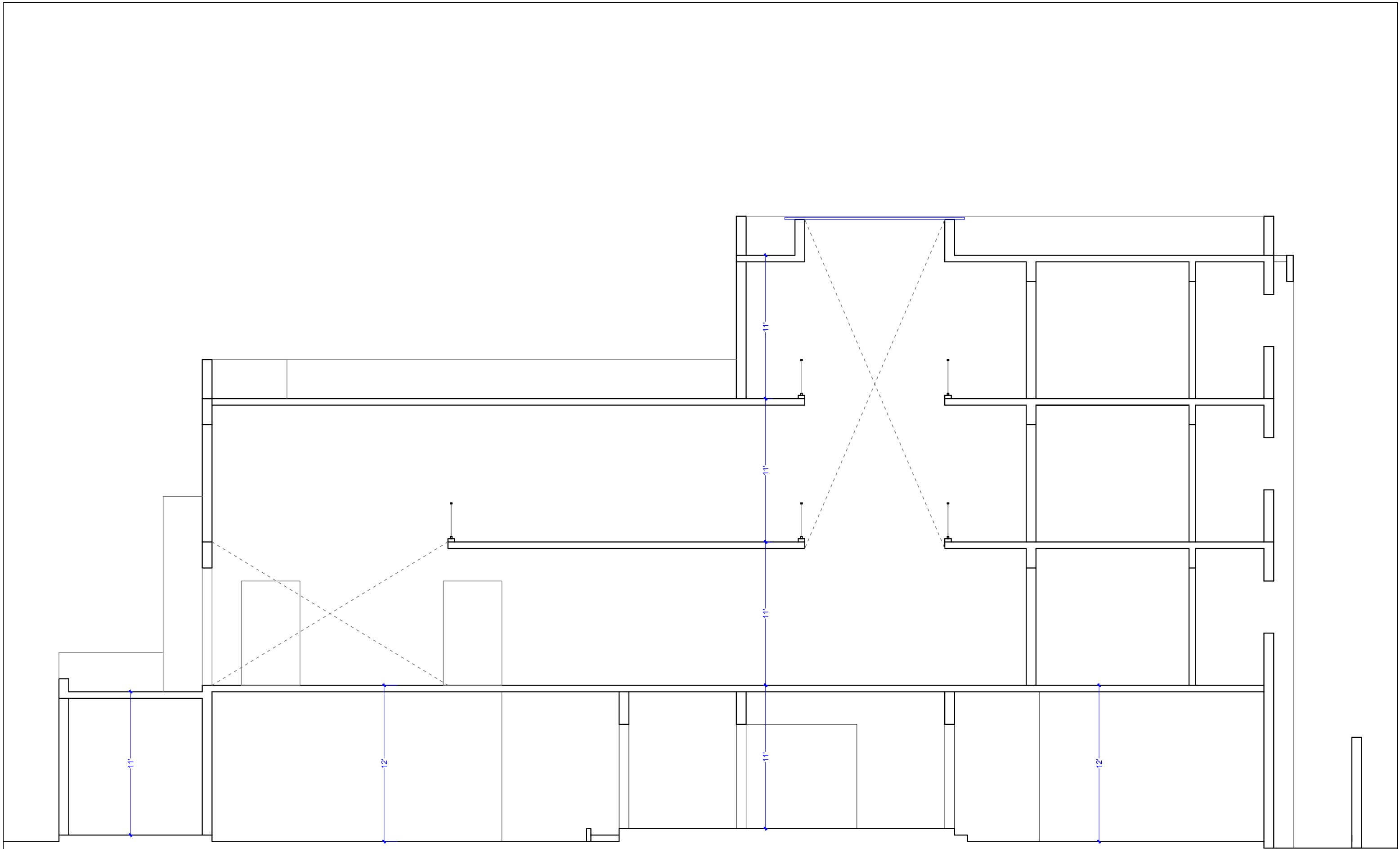
SECTION B-B'
